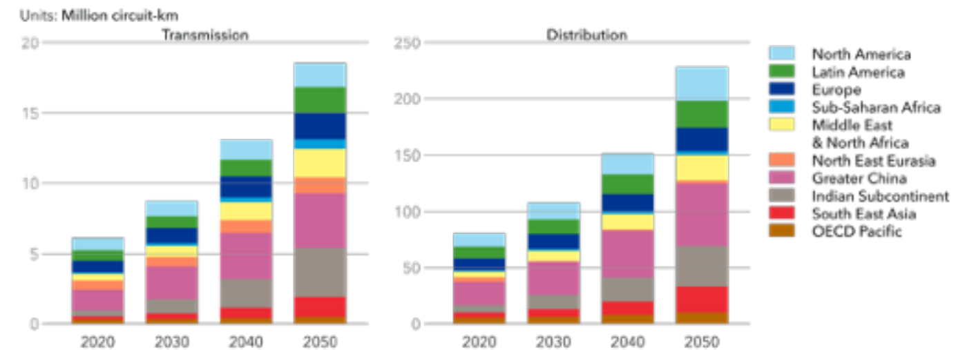
FIGURE 2.8 Transmission and distribution power-line length by region
