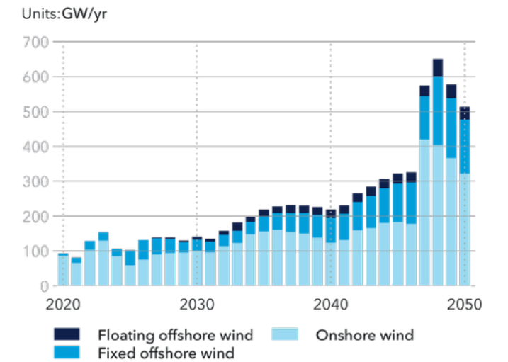
Wind gross capacity additions - PNZ
