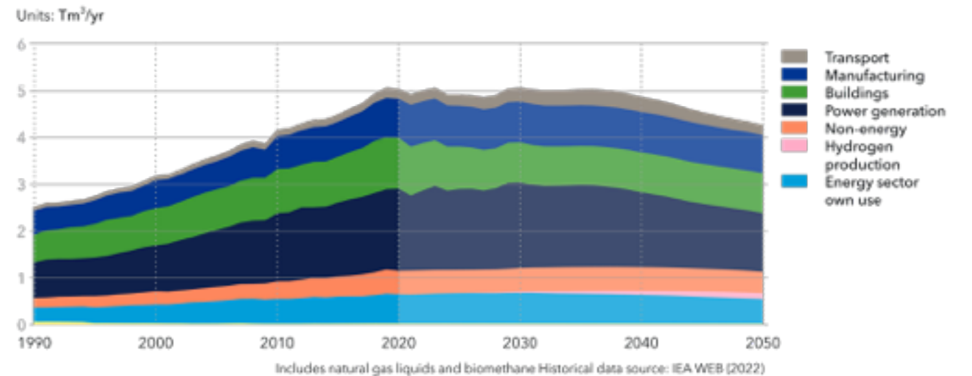
World natural gas demand by sector
