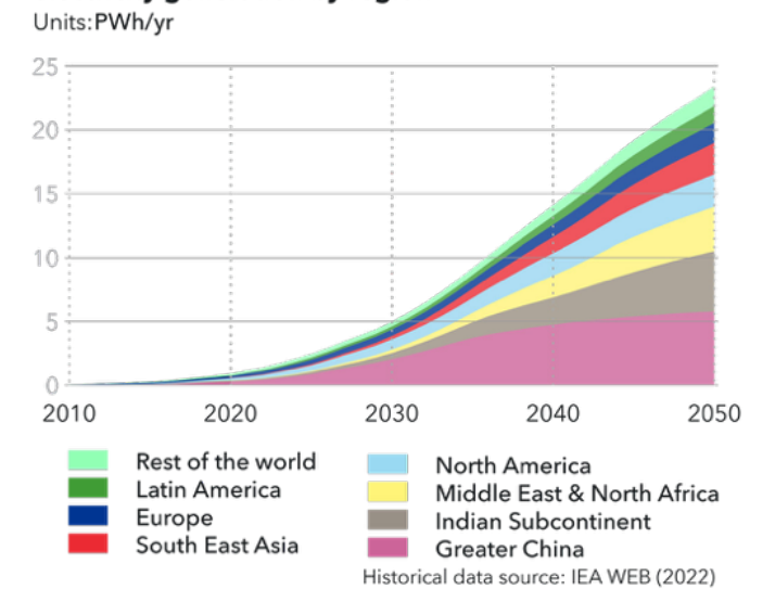
FIGURE 3.6 Grid-connected solar PV and solar+storage electricity generation by region
