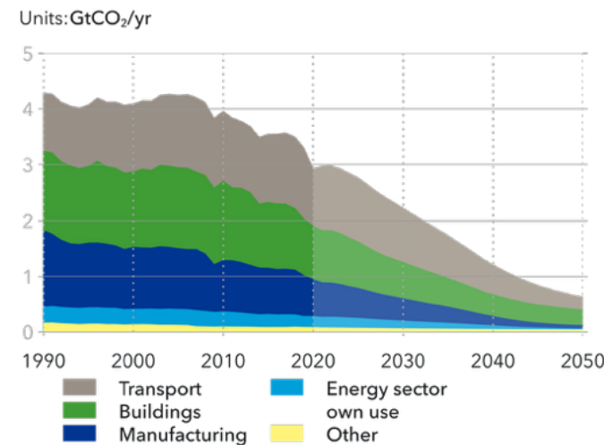
FIGURE 9.3.11 Europe energy-related CO 2 emissions by sector
