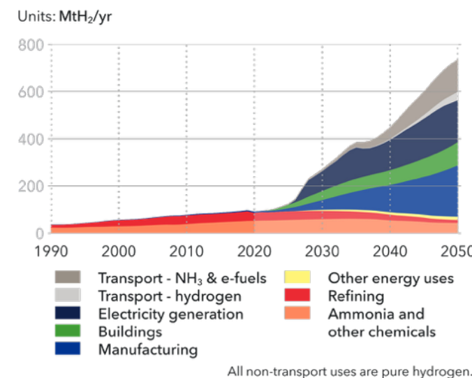
Global demand for hydrogen and its derivatives by sector - PNZ
