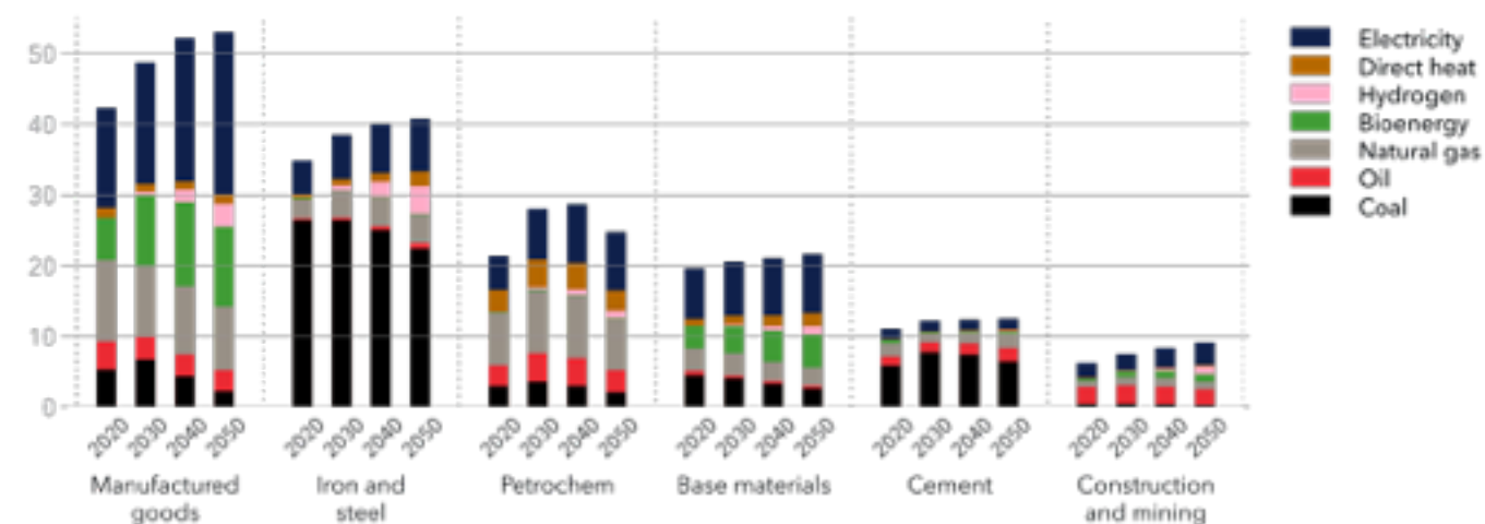
Manufacturing energy demand by subsector and energy carrier
