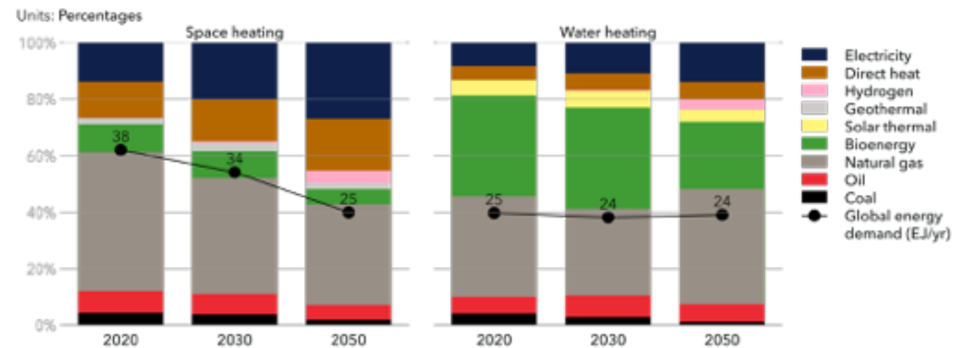
Space heating and water heating energy demand by carrier
